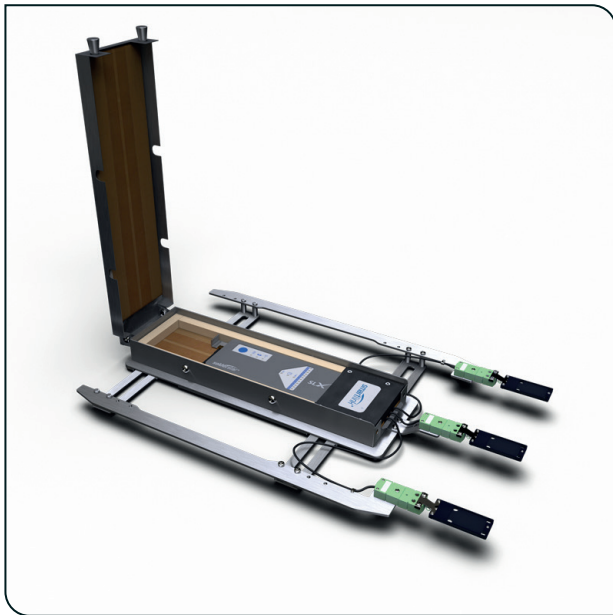
Adjustable fixture with matched oven performance sensors
